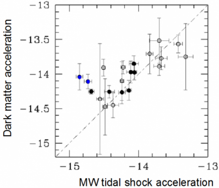
Caption : The gravitational acceleration of the dark matter believed to be in dwarf galaxies, as a function of that due to the tidal effects induced by the Milky Way. The dotted line shows where these two quantities are equal. The points indicate measurements on 21 dwarf galaxies. Credit: Observatoire de Paris - PSL/ Hammer et al. 2019
