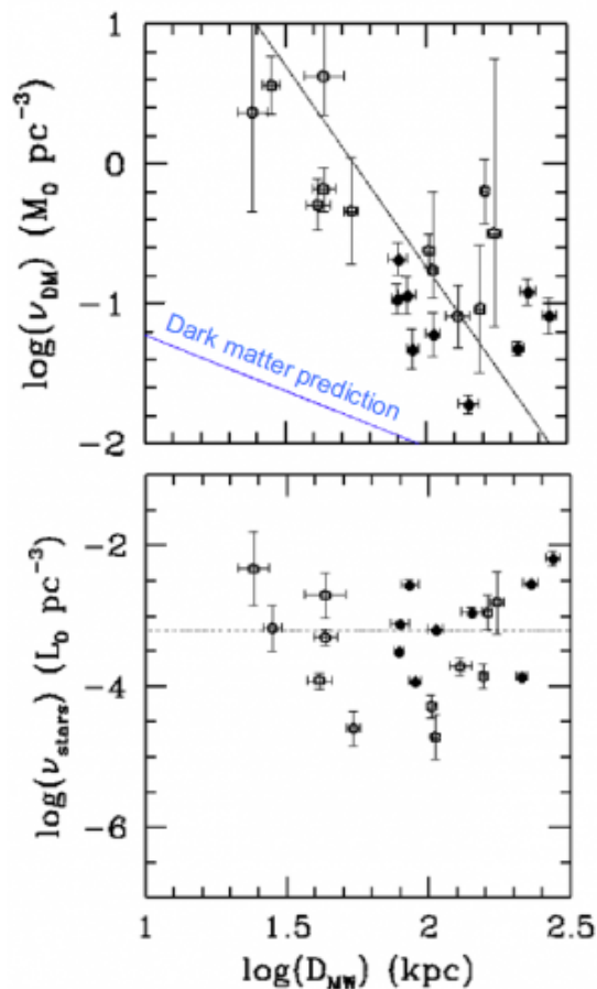
Caption : (Top panel) : the density of the hypothetical dark matter as shown by observations, which predict that it decreases significantly towards the outer regions of the Milky Way. The full line shows the loss of correlation with distance to the centre, the blue line shows the prediction of the dark matter model. (Bottom panel) : the stellar density
